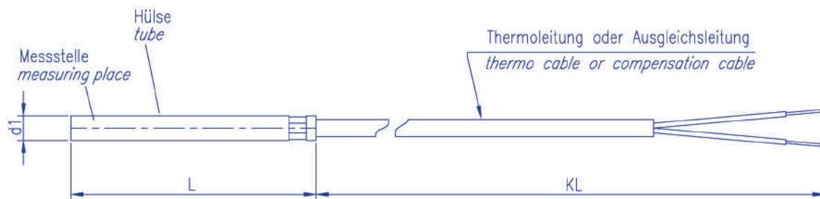
Hülsenthermoelement Sleeve thermocouple
